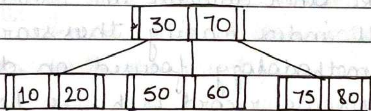
B-Tree
